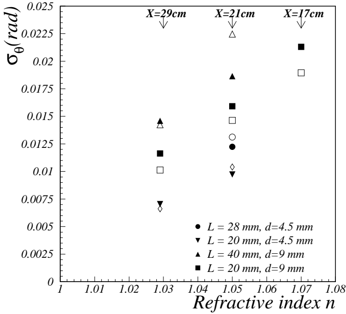
Fig. 5. The resolution i.e. the standard deviation of the single Cherenkov photon angular distribution for different values of the detector parameters, for a 3 GeV/c pion beam. Full symbols correspond to the measured values, empty ones to estimates of contributions from pixel size and emission point uncertainty only. X is the radiator-to-photon-detector distance, L is the radiator thickness and d is the photon detector pixel size.
