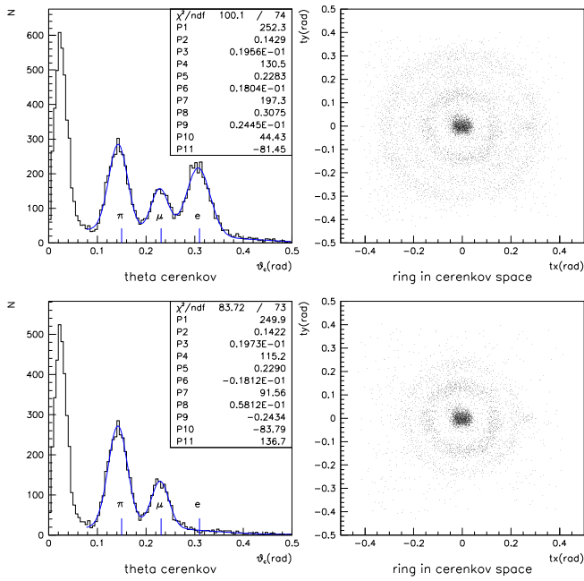
Fig. 4. Accumulated distributions of hits depending on their Cherenkov angle for all 0.5 GeV/c beam particles (top), and with gas Cherenkov signal vetoing the electrons (bottom). Aerogel with n = 1.05 was employed as the radiator.
