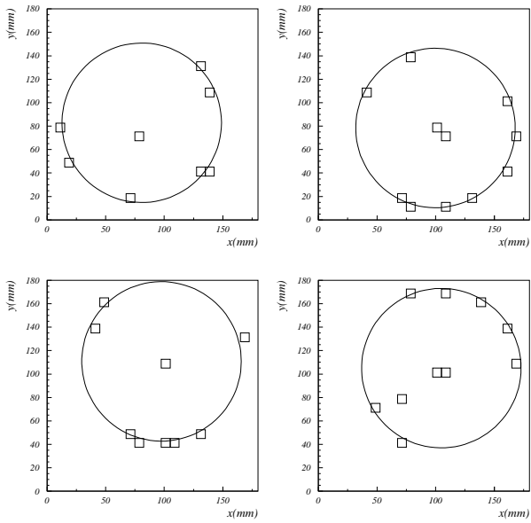
Fig. 2. Some examples of event hit patterns. The circle corresponds to the Cherenkov ring of 3 GeV/c pions given by the measured track position.
