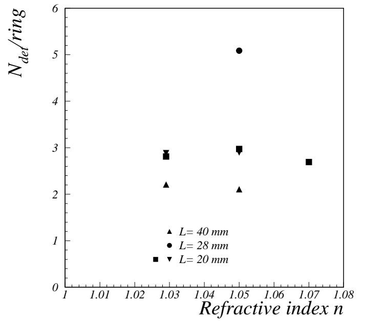
Fig. 6. Number of detected photons per Cherenkov ring for different aerogels, for a 3 GeV/c pion beam. L is the aerogel radiator thickness.
