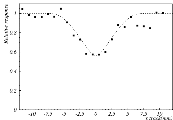
Fig. 8. The number of Cherenkov photons detected on the ring, as a function of the charged particle impact point distance from the side wall of the aerogel tile. The values shown are normalized to the measured values in case of a single tile covering the full range. Also shown is the estimate of a simple model.
