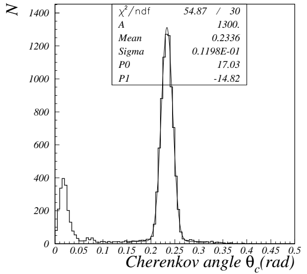
Fig. 3. Accumulated distributions of hits depending on their Cherenkov angle for 3 GeV/c pions, and n = 1.03 aerogel radiator.
