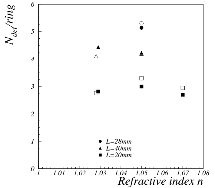
Fig. 6. Number of detected photons per Cherenkov ring for different aerogels, for a 3 GeV/c pion beam. L is the aerogel radiator thickness. Full symbols correspond to the measured values, empty ones to estimates.
