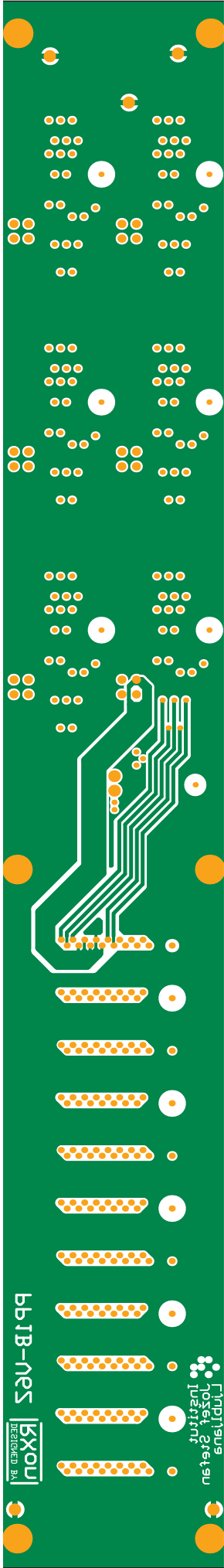
Layer 8 (Bottom)
