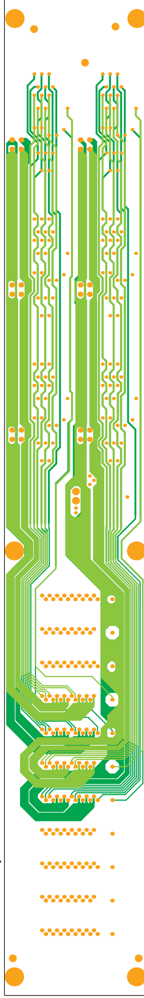
Layers 5 & 6
