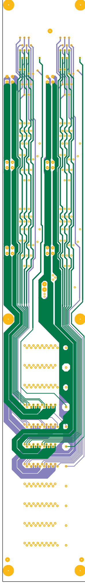
Layers 5 & 6
