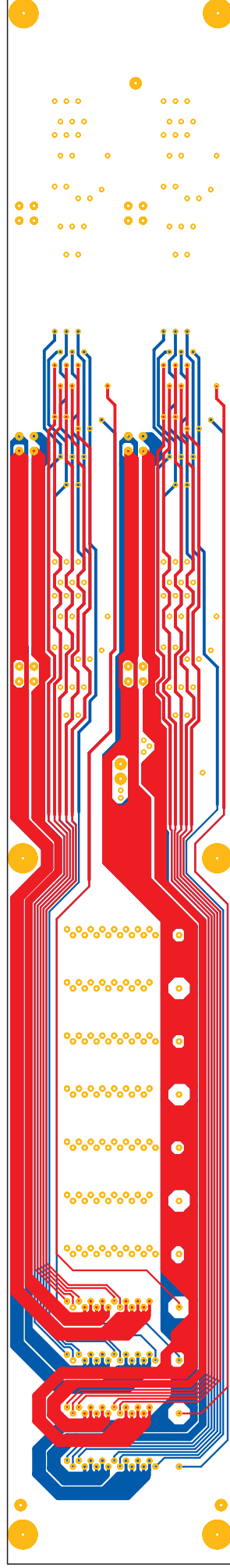
Layers 3 & 4
