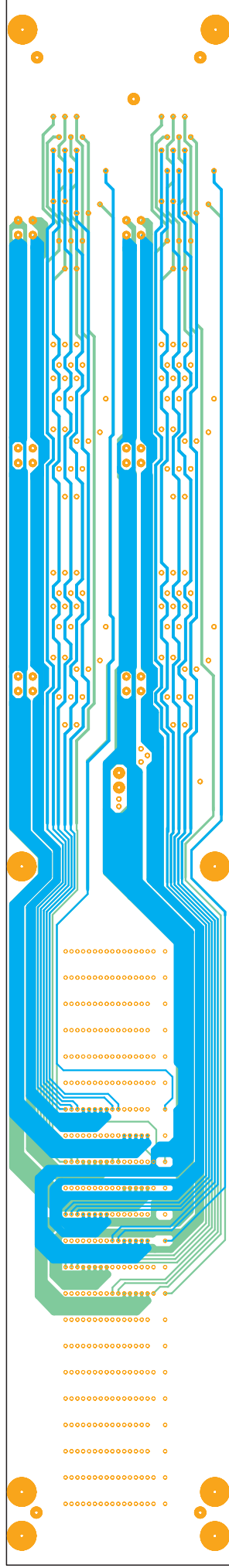
Layer 1-P (Top, Positive)
