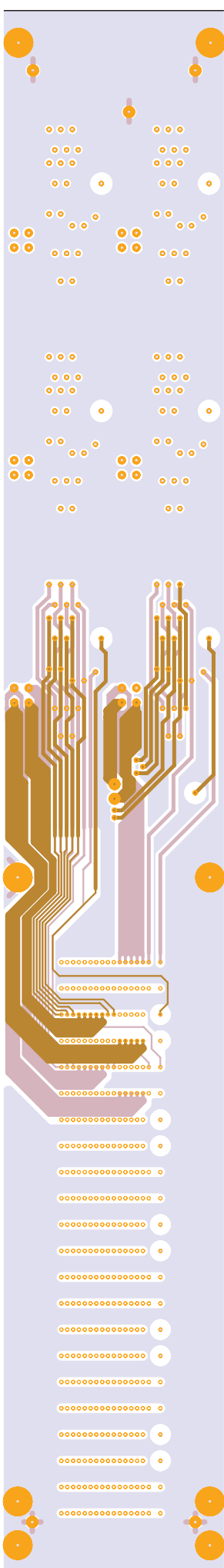
Layer 2-P (Positive)
