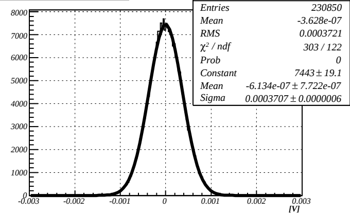
Noise, HV=1000V 200MHz
