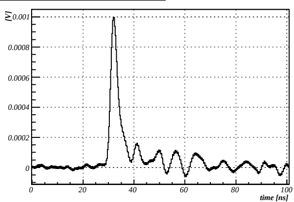
Average event, HV=1000V, 200MHz
