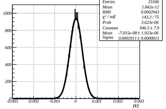
Noise, HV=600V
