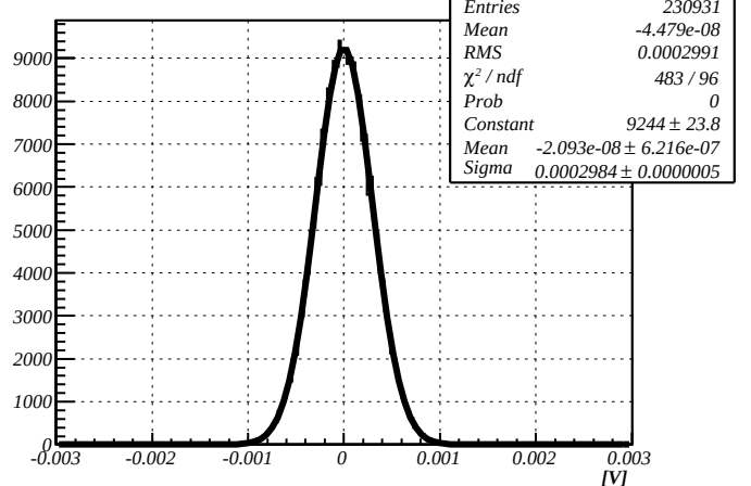
Noise, HV=1000V
