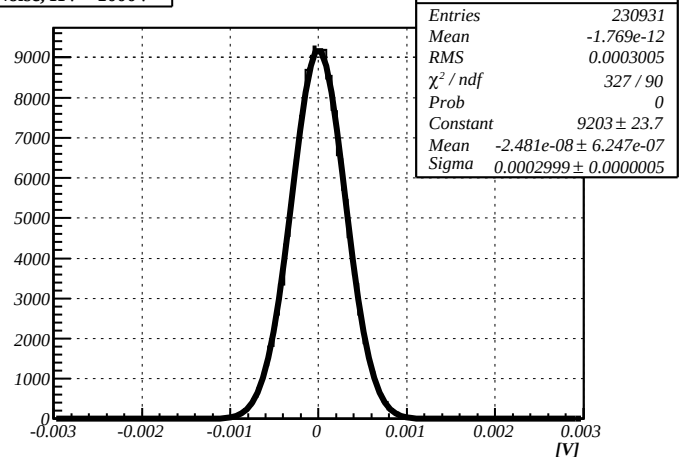
Noise, HV=-1000V
