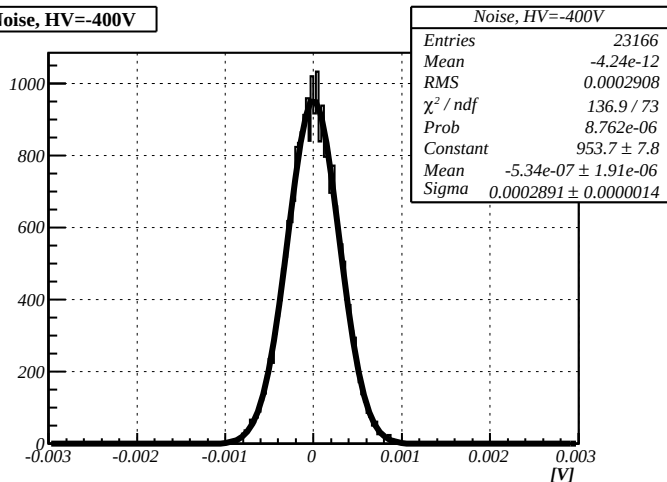
Noise, HV=-400V
