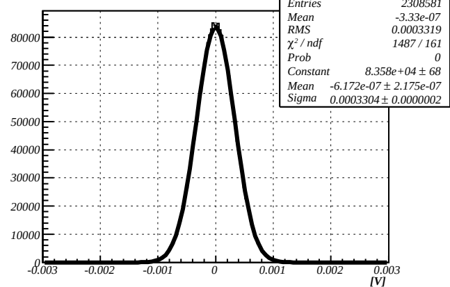
Noise, HV=1000V 200MHz
