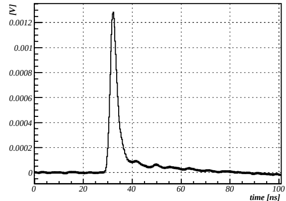
Average event, HV=1000V, 200MHz
