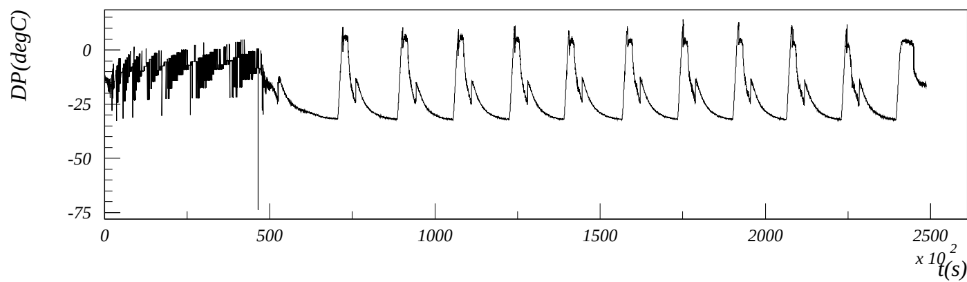
F405 and F424 Thermal Cycling
