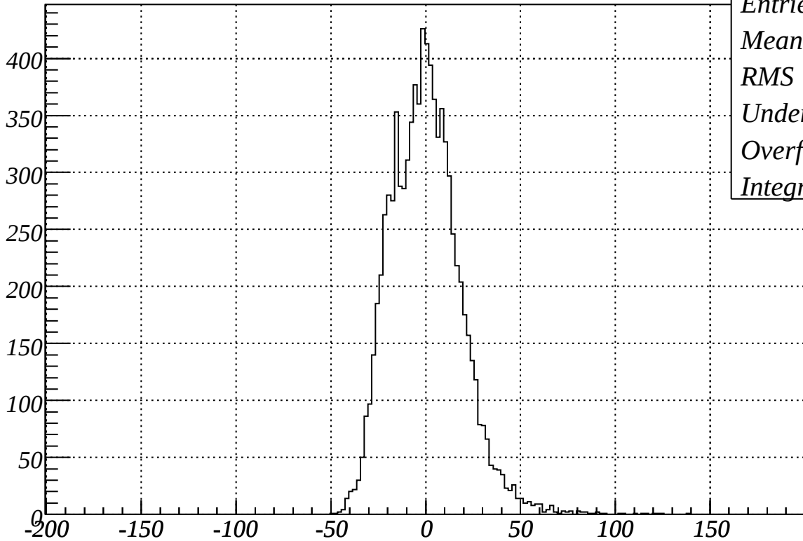
F403@-1000V, T11 setup2 CH1, noise
