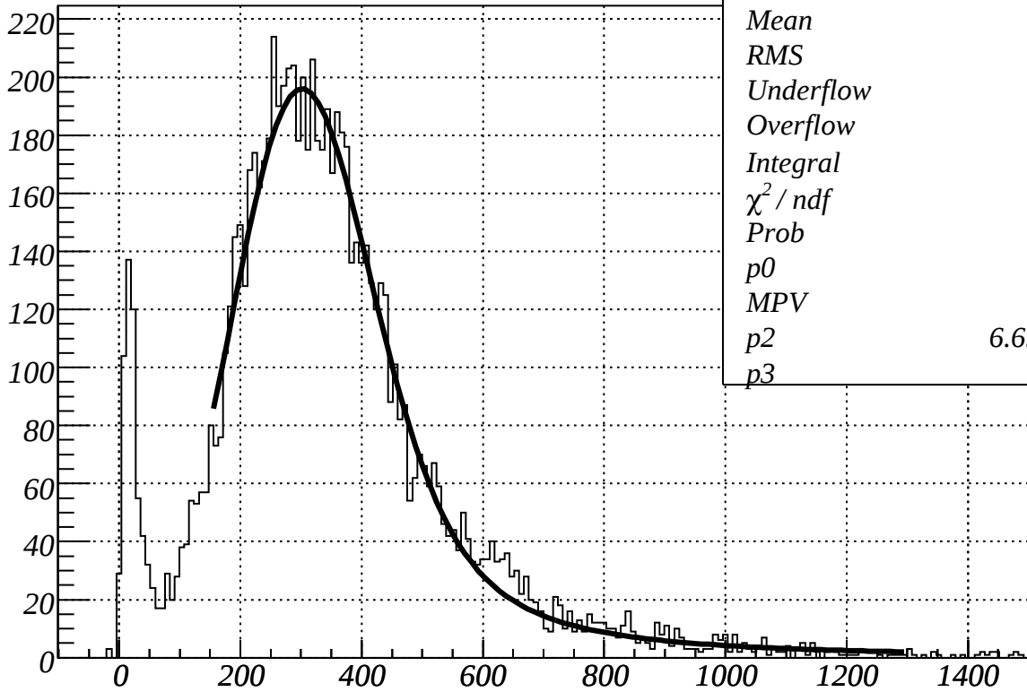
F403@-1000V, T11 setup2 CH1, signal
