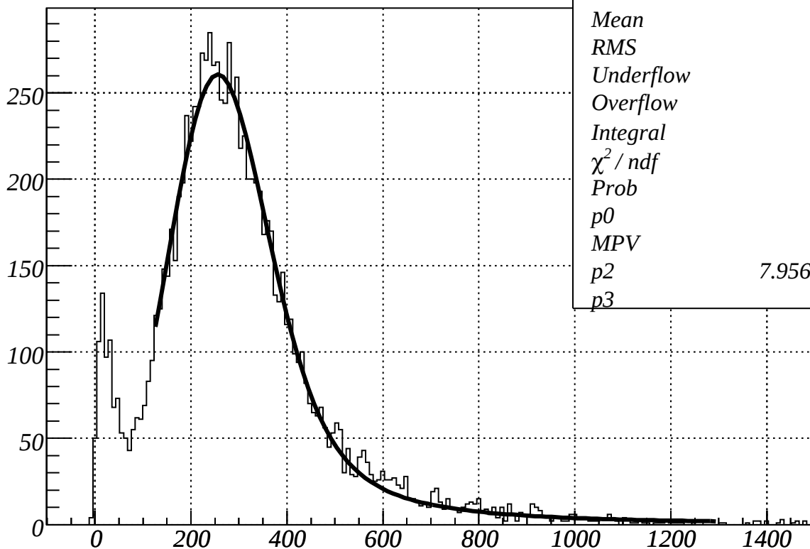
F404@+1000V, T11 setup1 CH2, signal
