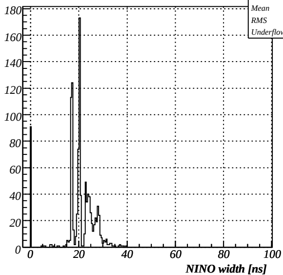
F404, setup2 T9, NINOthr=30.0mV
