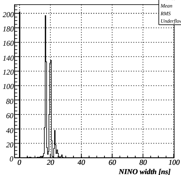
F404, setup2 T9, NINOthr=50.0mV
