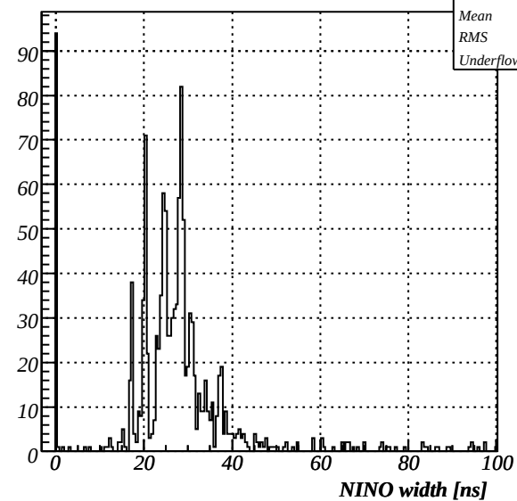
F404, setup2 T9, NINOthr=10.2mV
