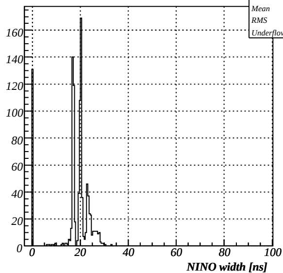
F404, setup2 T9, NINOthr=40.0mV
