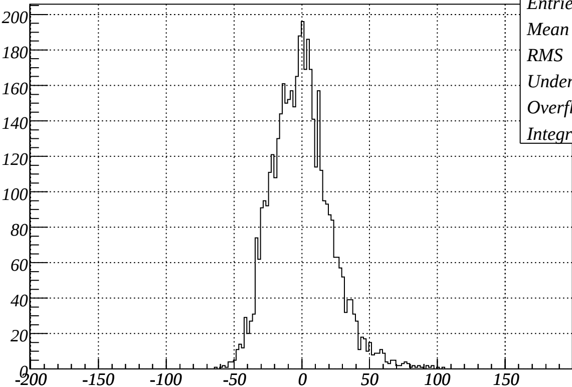
F405@+1000V, T9 setup5 CH3, noise
