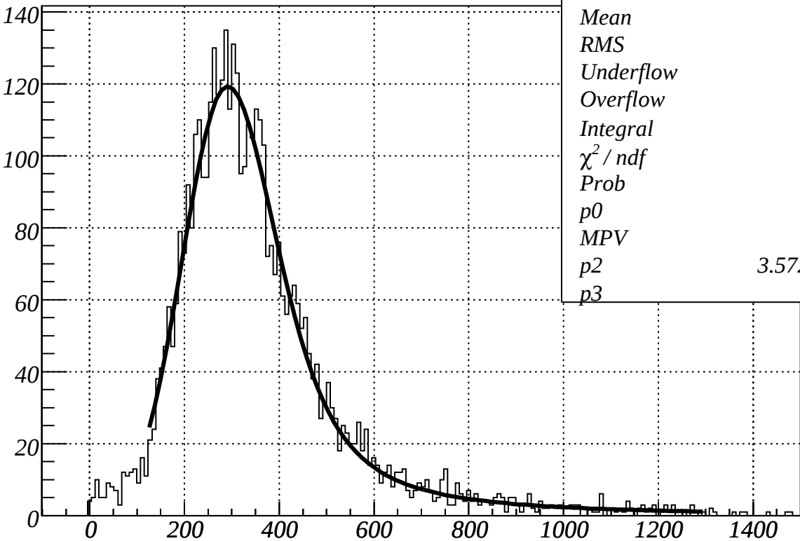
F405@+1000V, T9 setup5 CH3, signal
