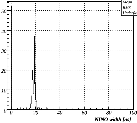
F405_setup2 T11, NINOthr=128.5mV
