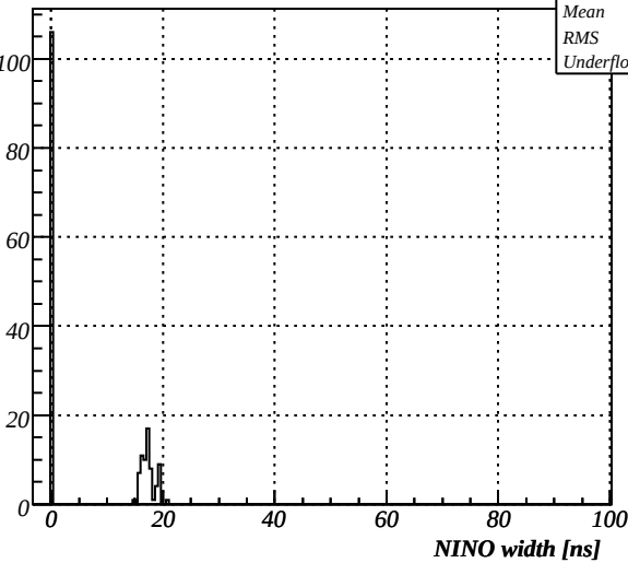
F405_setup2 T11, NINOthr=63.6mV
