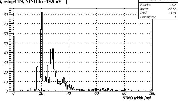
F406_setup4 T9, NINOthr=19.9mV
