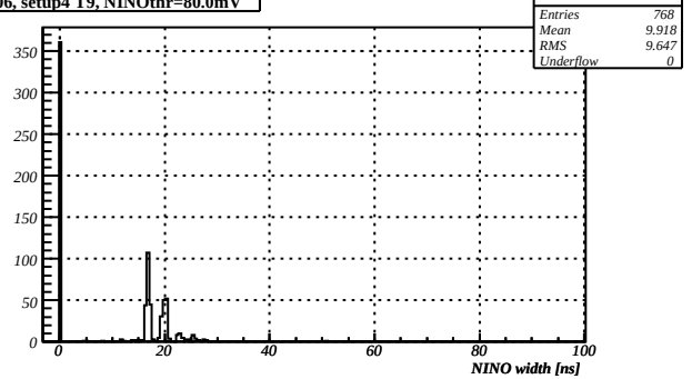
F406_setup4 T9, NINOthr=80.0mV
