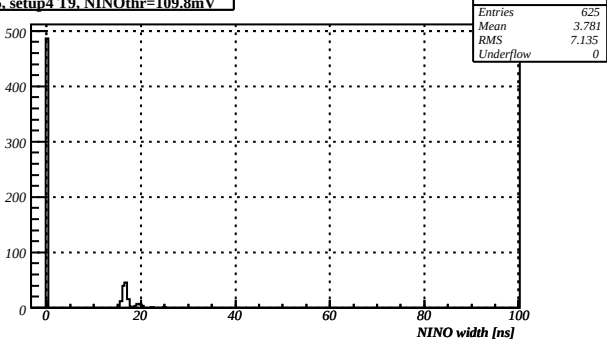
F406_setup4 T9, NINOthr=109.8mV
