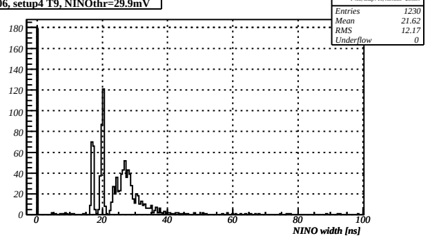
F406_setup4 T9, NINOthr=29.9mV
