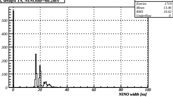
F406_setup4 T9, NINOthr=60.2mV
