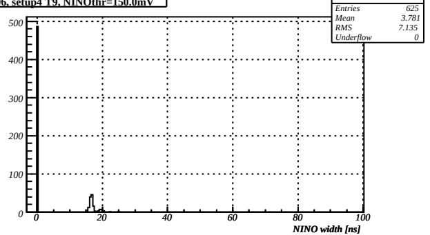
F406_setup4 T9, NINOthr=150.0mV
