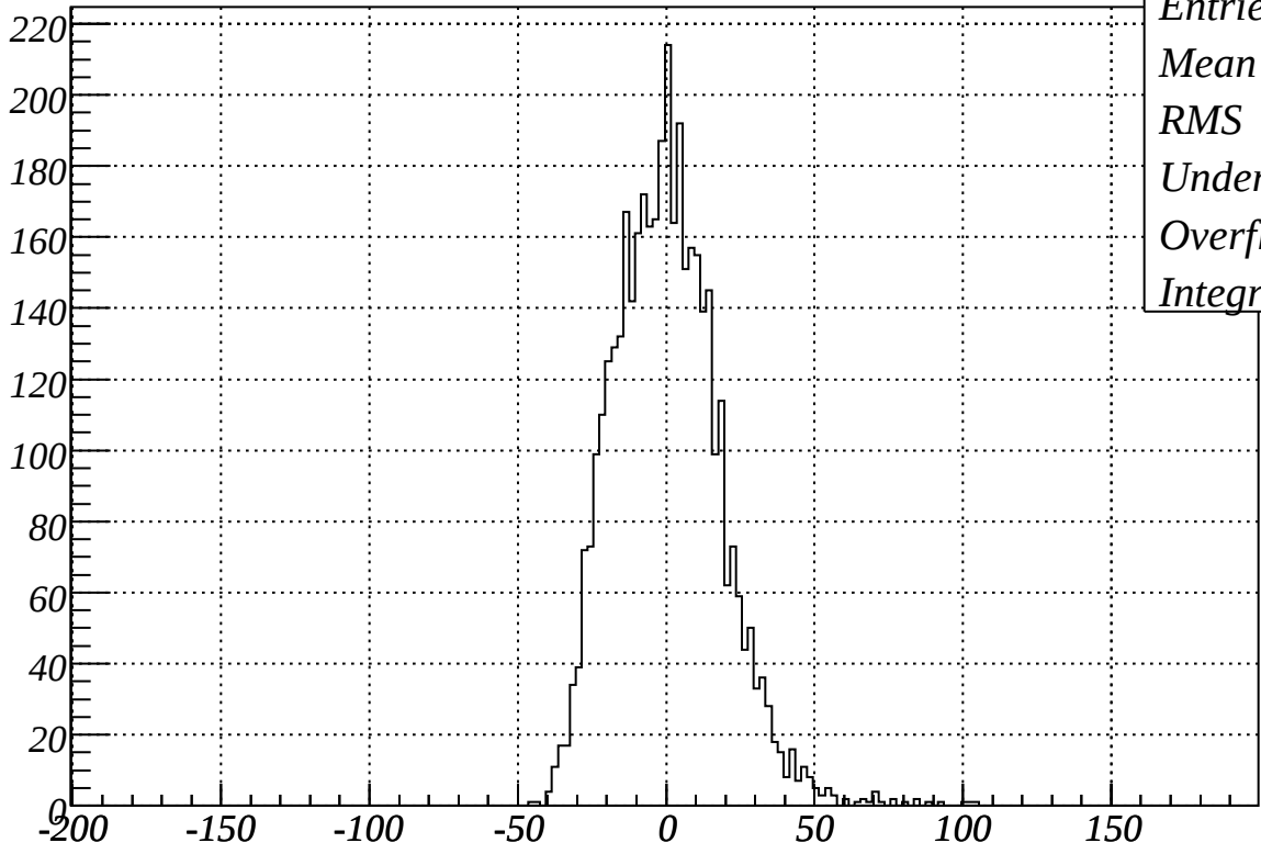
F407@-1000V, T9 setup3 CH1, noise
