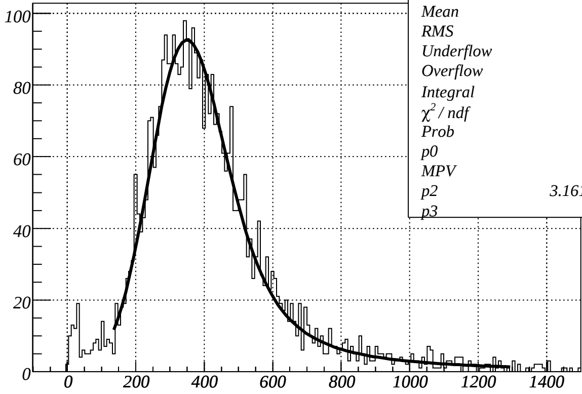
F407@-1000V, T9 setup3 CH1, signal
