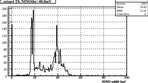
F407, setup4 T9, NINOthr=40.0mV
