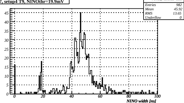
F407, setup4 T9, NINOthr=19.9mV
