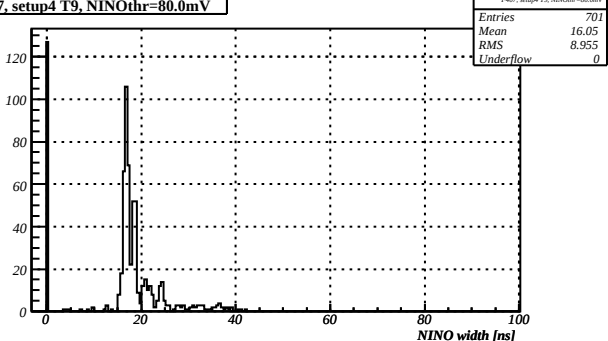
F407, setup4 T9, NINOthr=80.0mV
