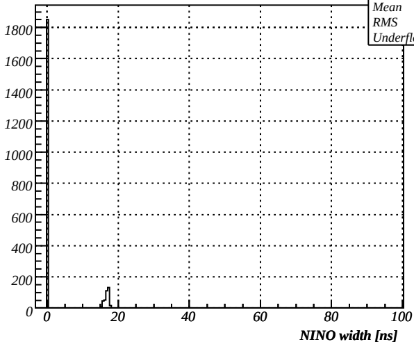
F408, setup5 T9, NINOthr=60.0mV
