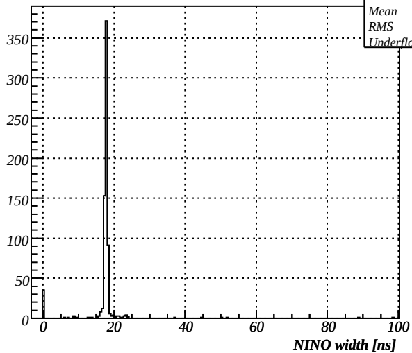
F409, setup3 T9, NINOthr=29.9mV
