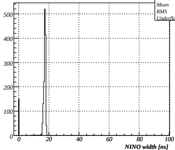
F409, setup3 T9, NINOthr=50.0mV
