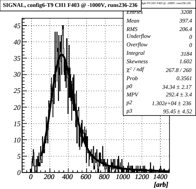
F403 config6-T9 CH1, runs236-236
