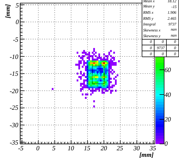
HIT MAP (sig>100.0), config6-T9 CH1 F403 @ -1000V, runs236-236
