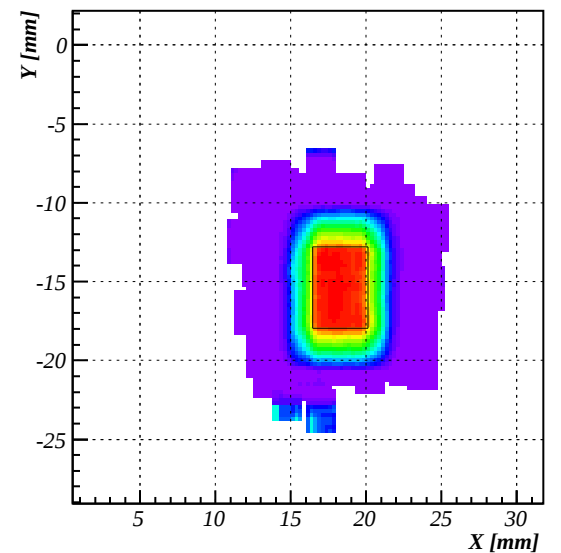
config6-T9 CH1 F403@-1000V, runs236-236, Efficiency(cut@100.0)
