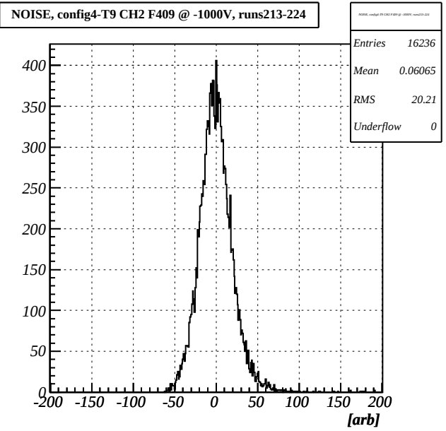
F409 config4-T9 CH2, runs213-224
