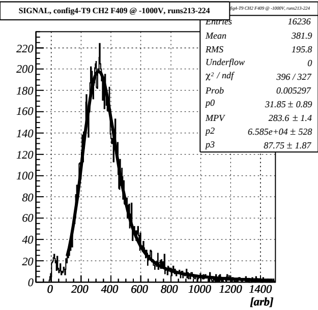
F409 config4-T9 CH2, runs213-224
