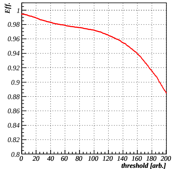
F409 config4-T9 CH2, runs213-224
