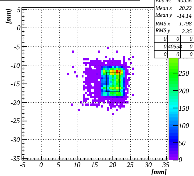
HIT MAP (sig>100.0), config4-T9 CH2 F409 @ -1000V, runs213-224
