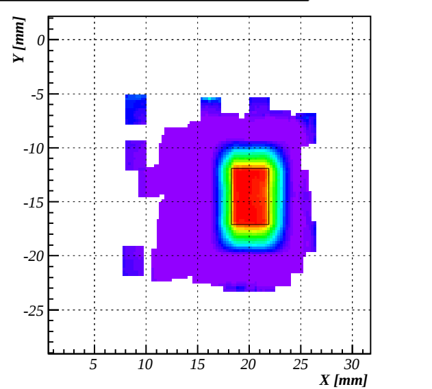
config4-T9 CH2 F409@-1000V, runs213-224, Efficiency(cut@100.0)
