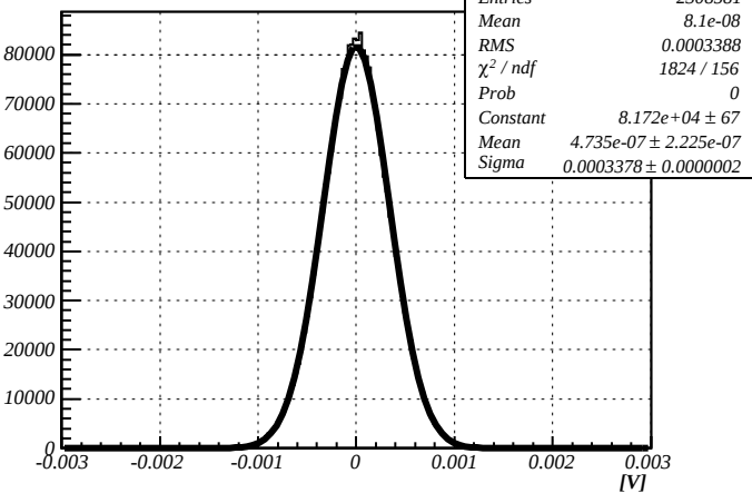
Noise, HV=-1000V
