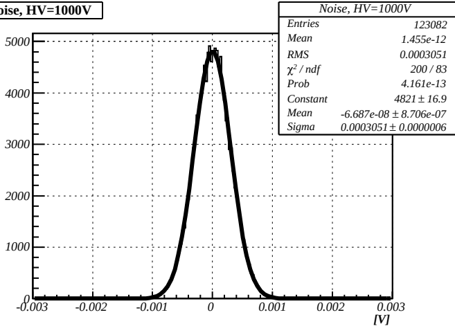
Noise, HV=1000V
