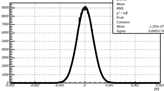
Noise, HV=1000V
