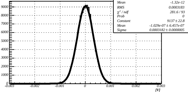
Noise, HV=1000V
