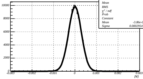
Noise, HV=1000V
