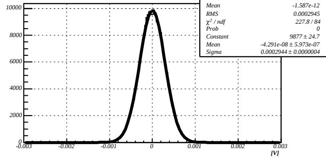
Noise, HV=1000V
