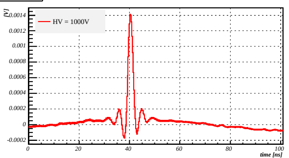
Average event
