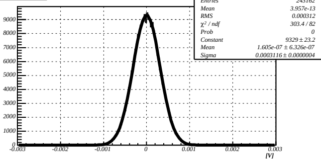
Noise, HV=1000V
