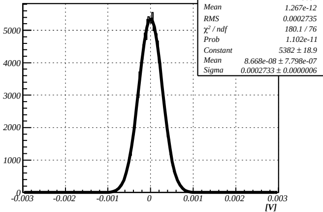
Noise, HV=1000V
