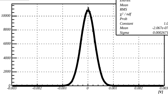
Noise, HV=1000V
