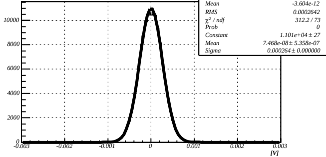
Noise, HV=1000V
