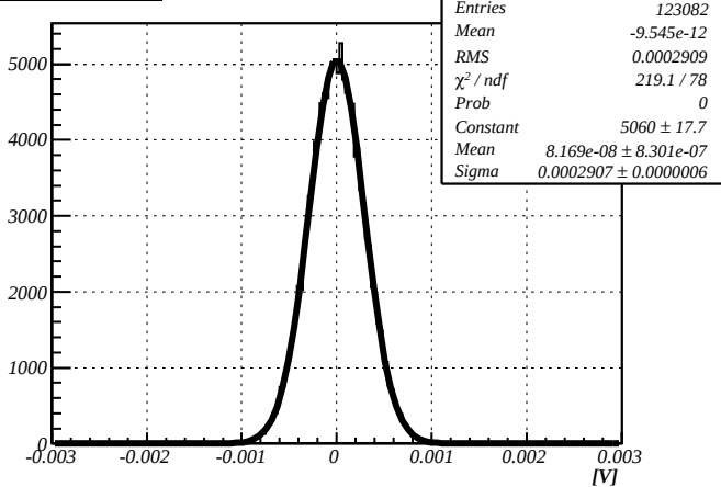
Noise, HV=1000V
