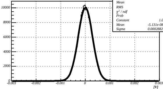
Noise, HV=1000V
