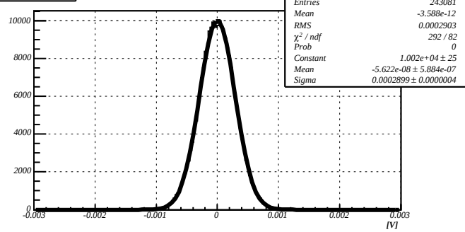
Noise, HV=1000V
