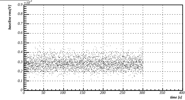
baseline rms
