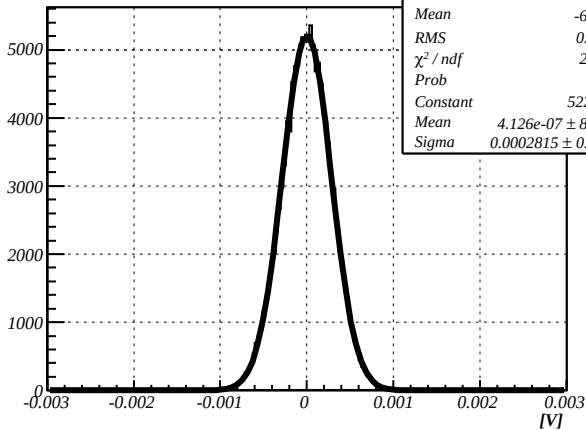
Noise, HV=1000V
