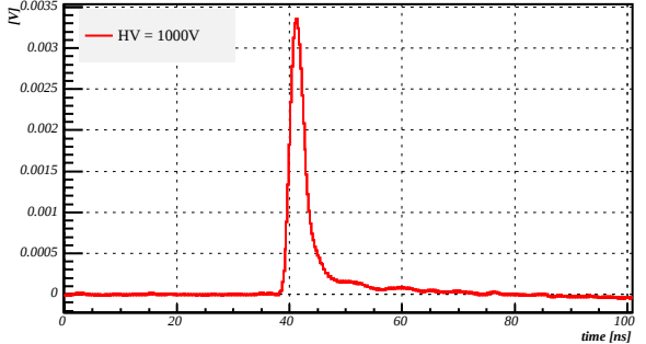
Average event
