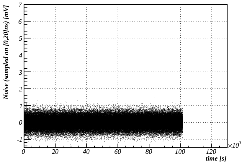
Noise sampled@10ns vs. time, CH215131, F413
