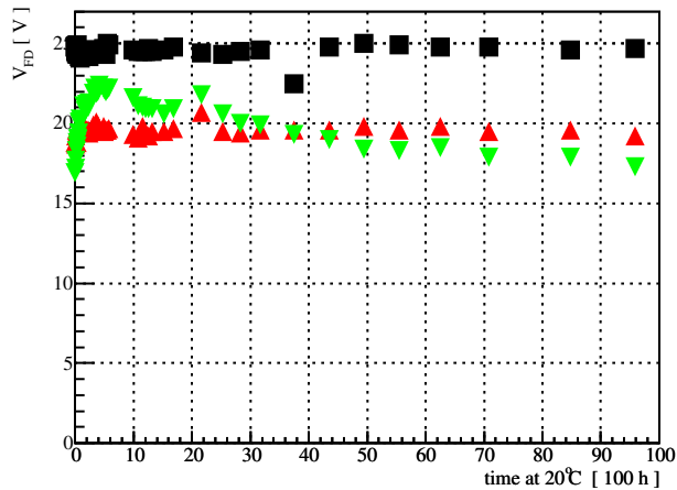
Full Depletion Voltage
