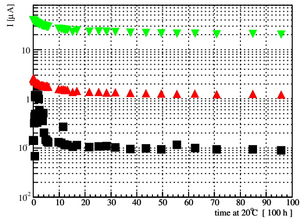
Leakage Current
