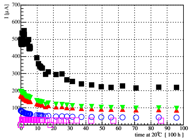
Leakage Current
