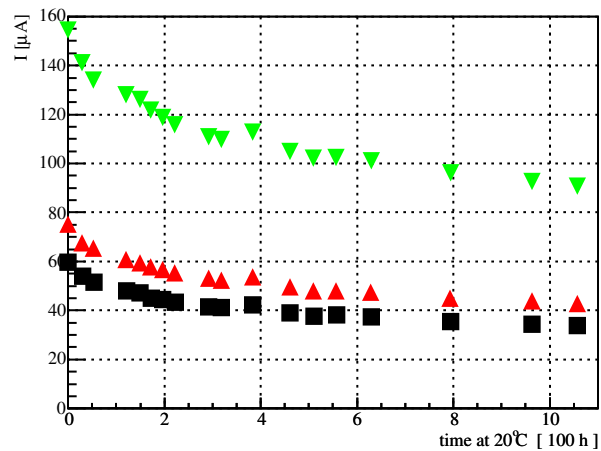
Leakage Current
