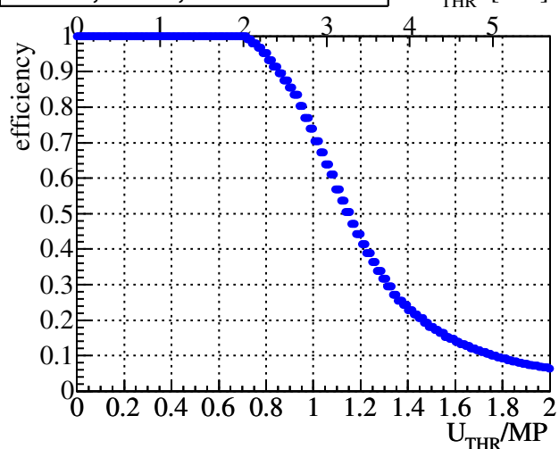
RUN=6, CH=1, 200MHz BWL
