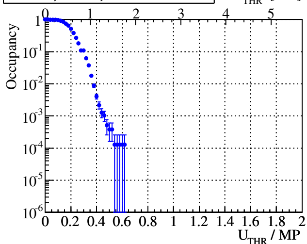
RUN=6, CH=1, 200MHz BWL
