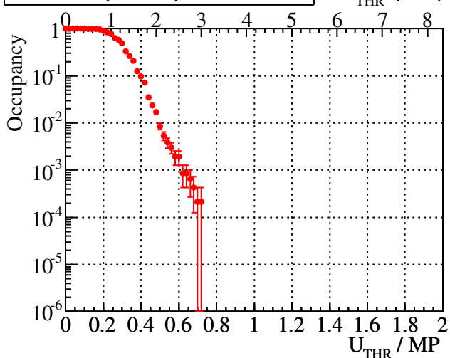
RUN=6, CH=1, No BWL
