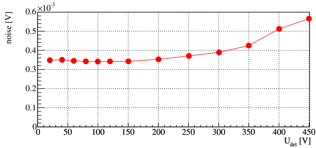
Noise
