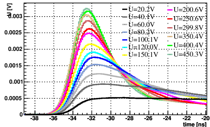
Averaged Histograms, run4,v01, 200MHz BWL
