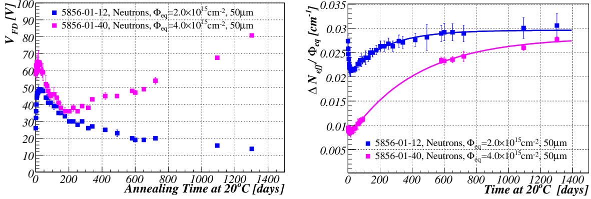
Figure 5.6: Examples of measured V_{FD} (left) as a function of annealing time at 20°C with corresponding \Delta N_{eff}/\Phi_{eq} annealing (right). The solid lines on the right plot represent the best fit of function 5.2 to calculated \Delta N_{eff}/\Phi_{eq} values.
