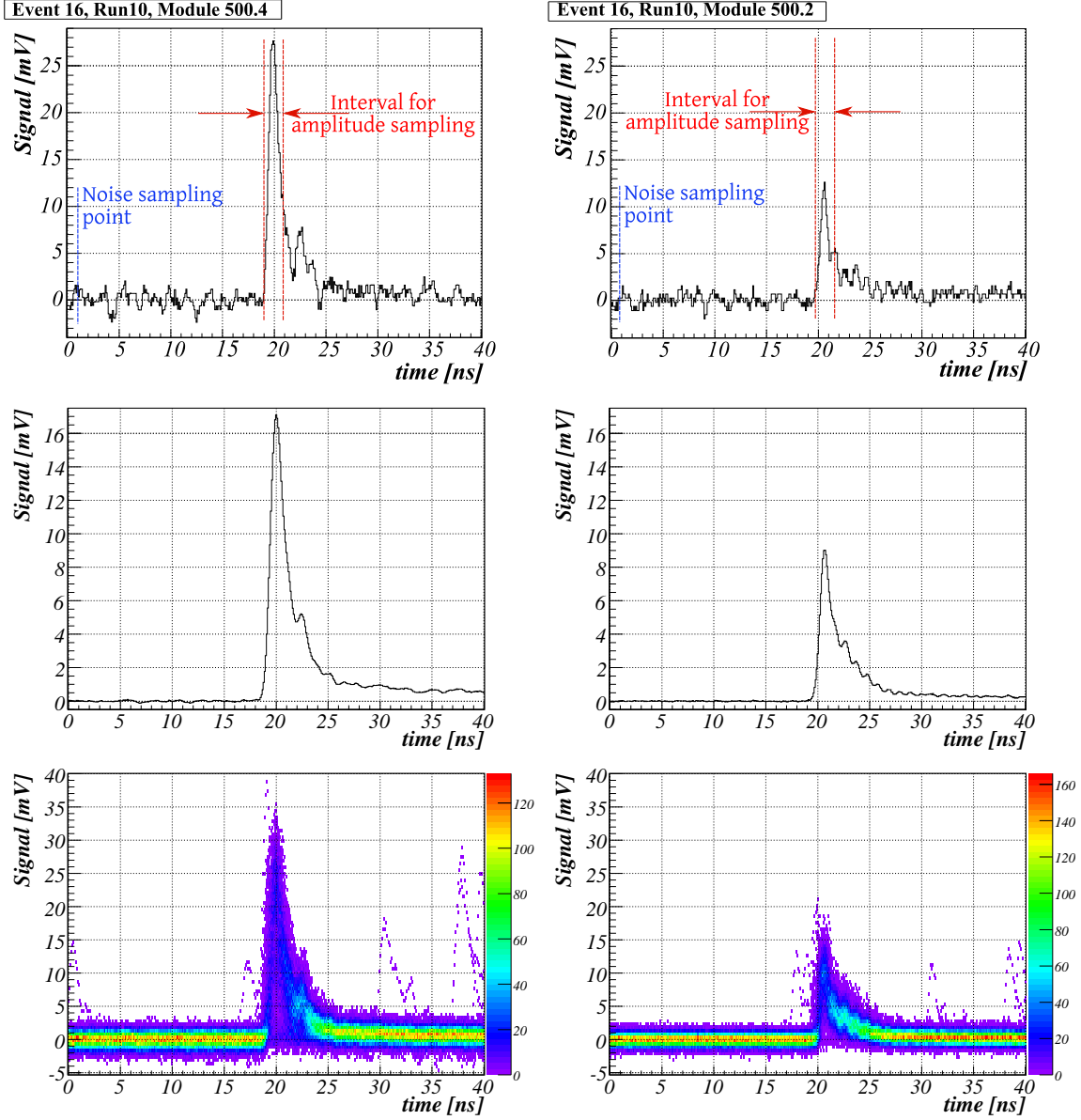
Figure 4.8: Single event (up), average waveform (middle) and two-dimensional histogram (bottom) containing all recorded waveforms (persistence plot) for module 500.4 (left), and module 500.2 (right), obtained from data run 10 ( \vartheta=45^\circ ).
