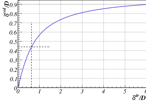
Figure 3.12: Charge collection distance \delta^{ccd} dependence on drift length \delta^{dr} , both in units of detector thickness. The dotted lines denote their values for diamond sensors used in this work. Assumptions leading to this dependence are discussed in text.
