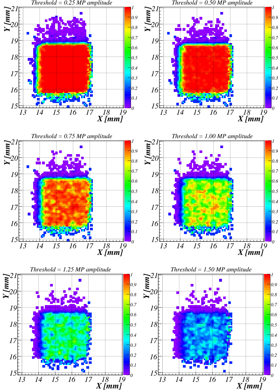
Figure 4.20: Efficiency of analogue signals scanned over the diamond area in steps of 0.1 mm for module F408 at -1000 V. Efficiency was calculated as the fraction of pion tracks in 0.2 \times 0.2 \text{ mm}^2 with signal amplitude higher than the threshold value in each step. The threshold values for each plot are given in units of MP amplitude. The plots were extracted from the data collected in H8 beam line when module was positioned as anticipated in ATLAS.
