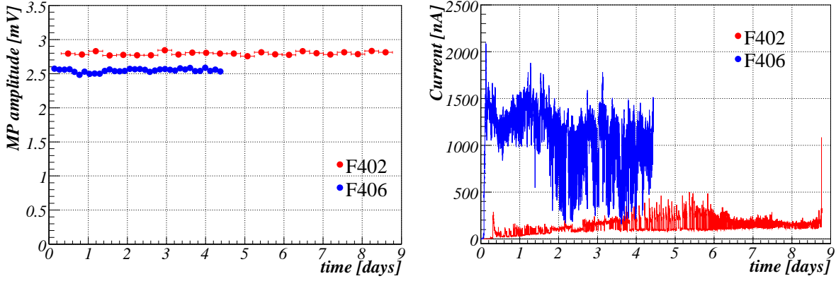
Figure 4.29: Long term behaviour of MP amplitude (left) and leakage current (right) measured at 2 \text{ V}/\mu\text{m} bias electric field for module F402 (red) and F406 (blue). MP amplitudes were extracted in time slices of 8.5h ( \sim 6500 events) for module F402 and 3h ( \sim 9000 events) for module F406.
