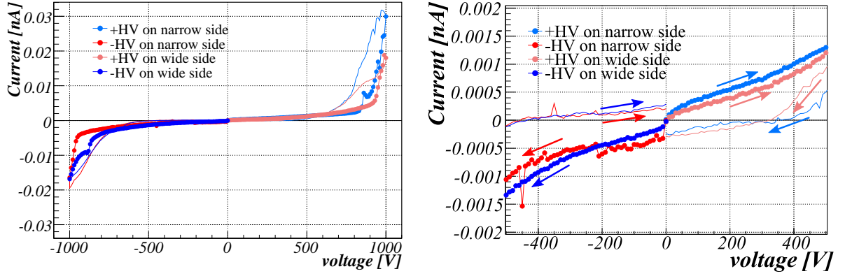
Figure 4.3: Left: Measured I–V characteristic for sample A382-11. Blue curves denote the measurements with more positive potential applied to the narrow side and red curves represent the case of more positive potential applied to the wide side. Note that for each colour light and dark curves should match, since they refer to the same direction of the electric field. Thick curves represent the ramping up from 0 V to \pm 1000 V, while the thin curves refer to ramping back down to 0 V. Due to polarisation effect the curves with and without markers do not match. The plot on the right shows a magnified part of plot on the left. The voltage ramping direction is marked by arrows.
