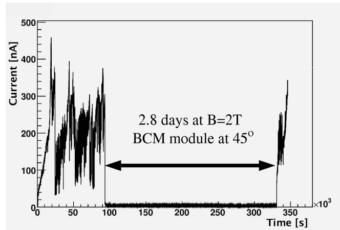
Figure 4.31: Leakage current of BCM detector module F408 at 1000 \text{ V} . After one day the module was placed in magnetic field of 2 \text{ T} for 2.8 days.
