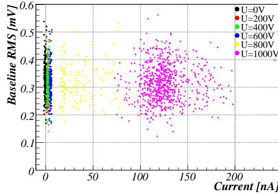
Figure 4.30: The RMS of baseline fluctuations, extracted for the recorded waveforms, as a function of BCM module current, measured during m1 voltage scan with module F402.
