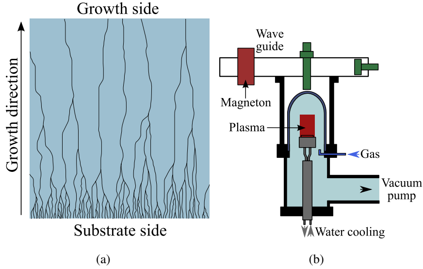
Figure 3.10: (a) Schematic side view of pCVD diamond sample. (b) Schematic picture of Microwave plasma CVD reactor.
