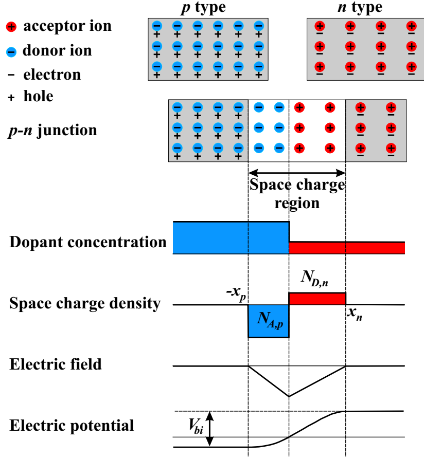
Figure 3.4: Dopant concentration, space charge density, electric field strength and potential of the p-n junction.
