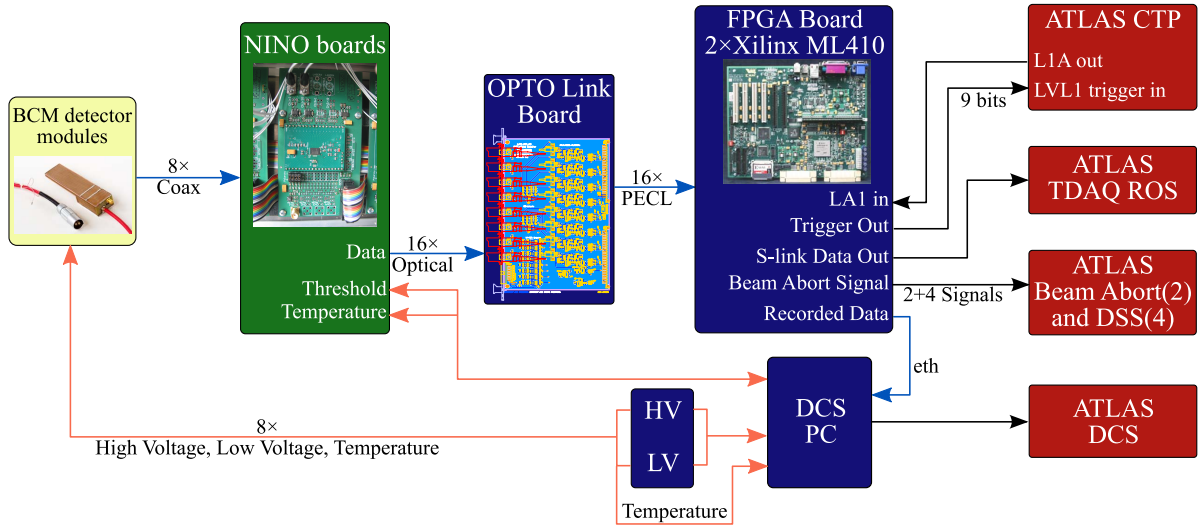
Figure 2.11: Overview of the BCM readout and supply chain.
