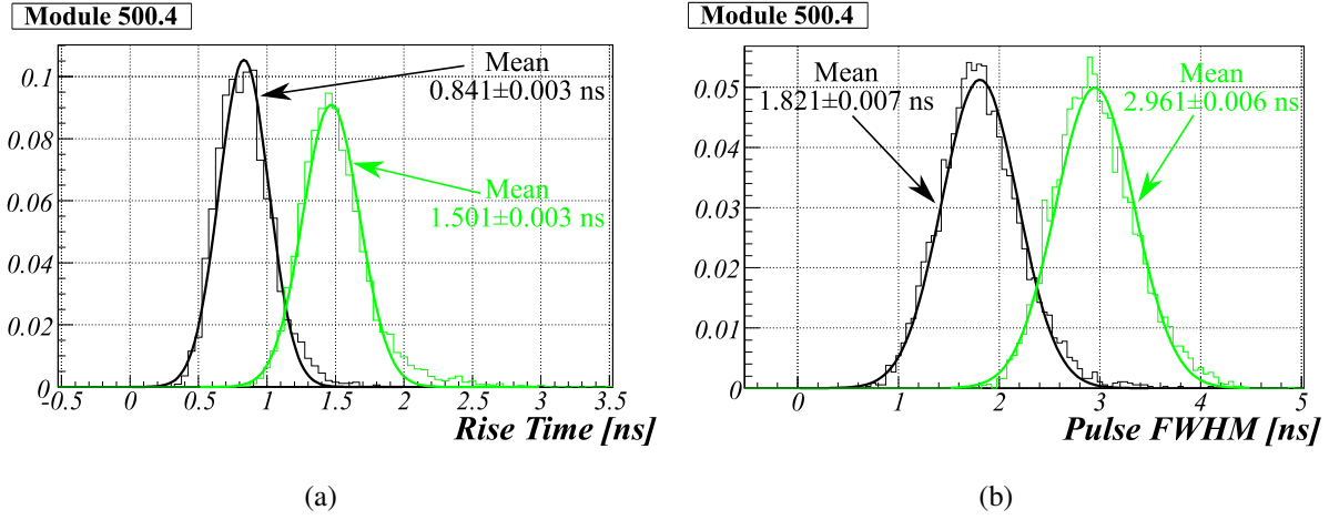
Figure 4.13: (a) Pulse rise time and (b) FWHM width distributions obtained for module 500.4 at 2 V/μm electric field and 1 GHz (black) or 200 MHz BWL. Mean of the distributions and its standard error are written on the plot.
