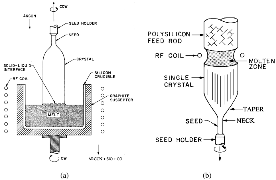
Figure 3.5: Schematic setup for (a) Czochralski and (b) Float zone process. Source [Sze02].
