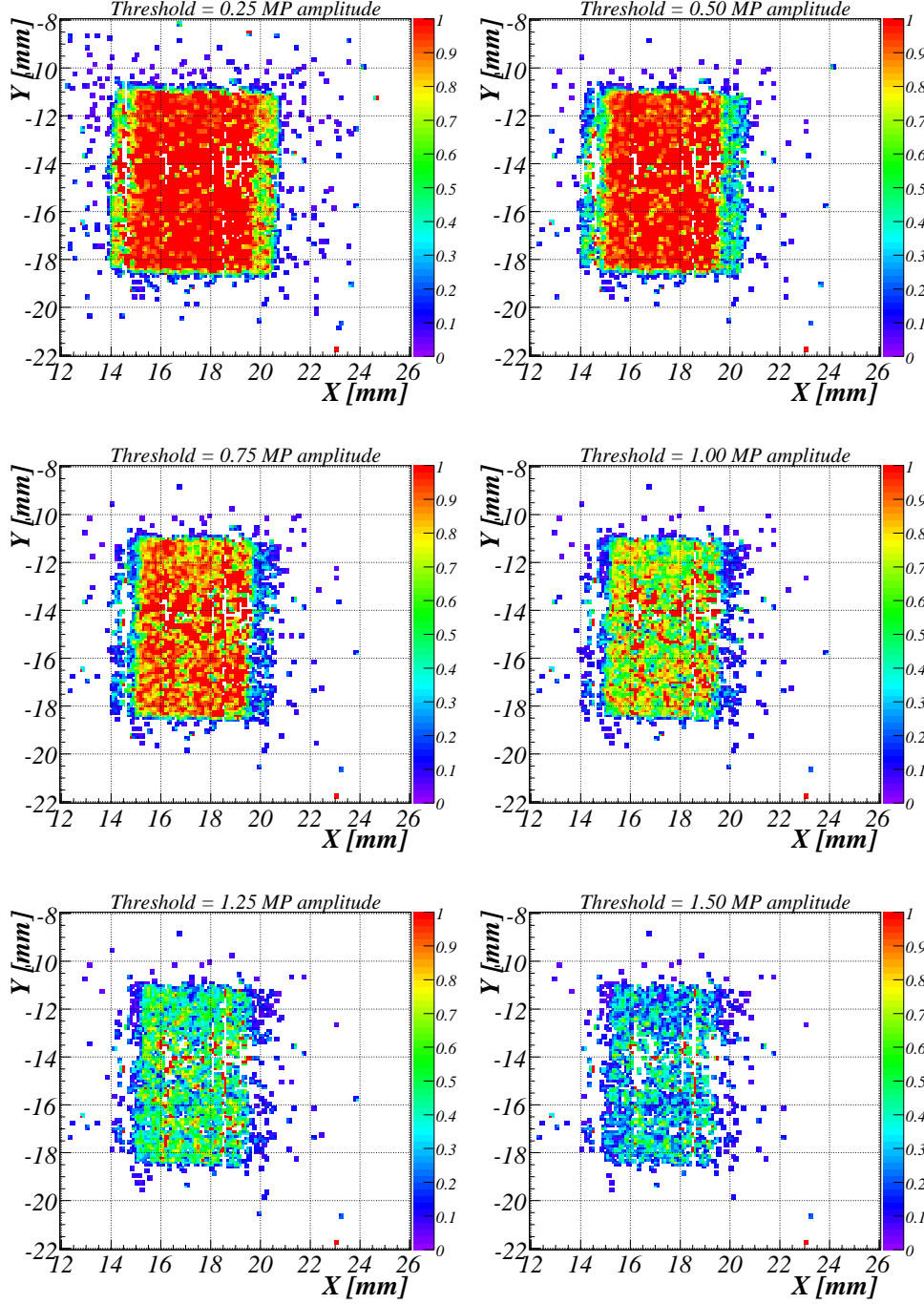
Figure 4.19: Efficiency of analogue signals scanned over the diamond area in steps of 0.1 mm for module F408 at +1000 V. Efficiency was calculated as the fraction of pion tracks in 0.2 \times 0.2 \text{ mm}^2 with signal amplitude higher than the threshold value in each step. The threshold values for each plot are given in units of MP amplitude. The plots were extracted from the T9 data where modules were not aligned with the beam as in ATLAS.
