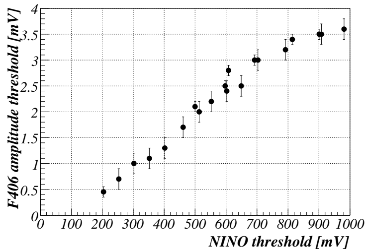
Figure 4.41: Correlation between NINO discriminator threshold and the threshold on the scale of NINO input signal amplitudes. The values have been estimated from the width-amplitude plots as shown in figure 4.42 obtained with module F406 and spare final NINO board.
