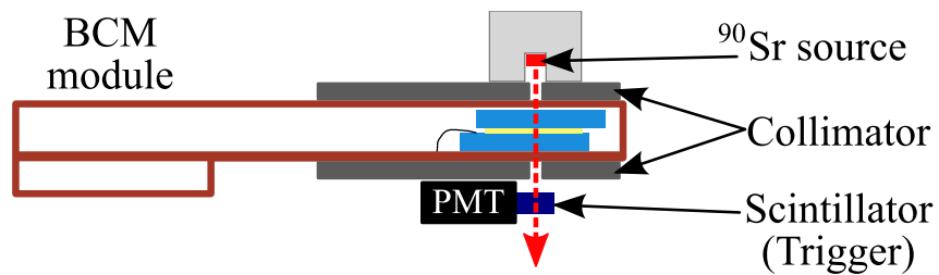
Figure 4.22: Schematic picture of the setup used for measurements with ^{90}\text{Sr} source.
