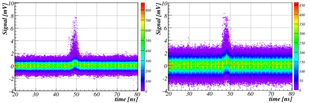
Figure 5.11: Two dimensional histograms of recorded waveforms with 50\text{ }\mu\text{m} epi sample at 450 V bias voltage for 200 MHz (left) and no BWL at readout.
