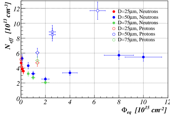
Figure 5.5: N_{eff} at the end of short term annealing as a function of equivalent fluence for proton (open markers) and neutron (closed markers) irradiated 25 \mu\text{m} (red), 50 \mu\text{m} (blue) and 75 \mu\text{m} (green) samples.
