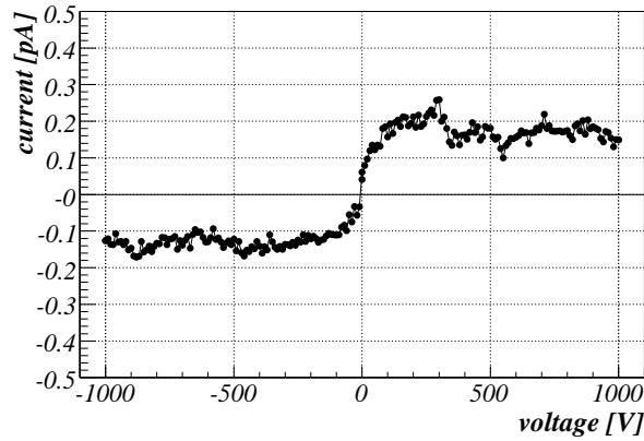
Figure 4.2: I–V measurement performed without a diamond sample.
