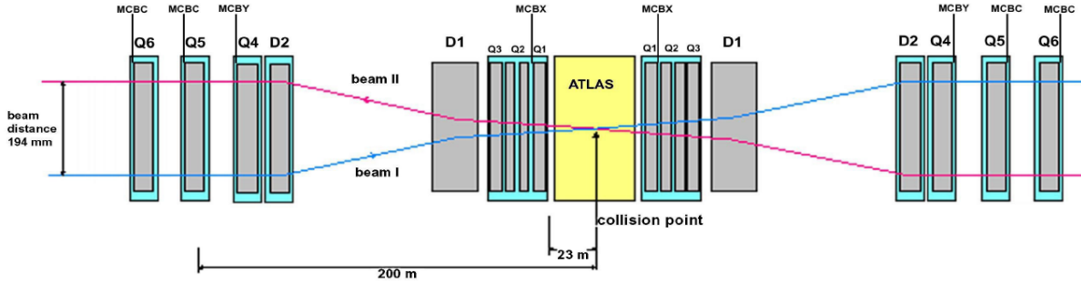
Figure 2.3: The ATLAS insertion region (IR1) beam optics.
