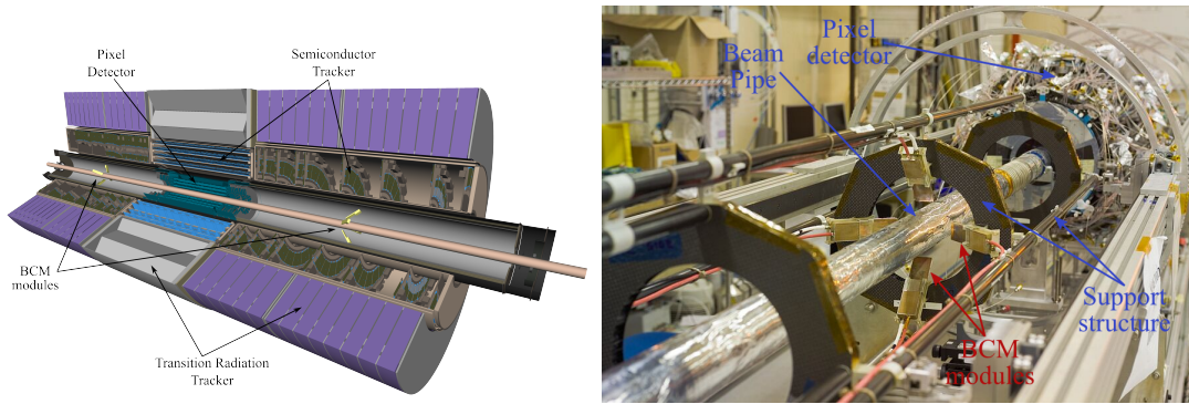
Figure 3: Position of detector modules inside ATLAS Inner detector (left). Modules are mounted on the Pixel support structure (right).
