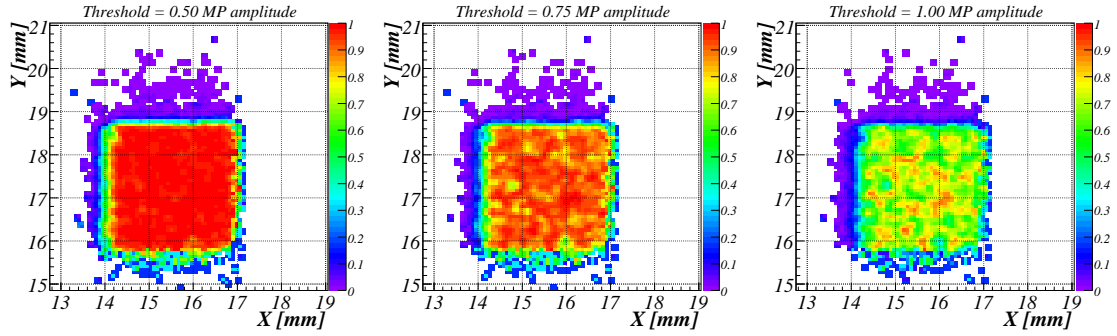
Figure 5: Efficiency of analogue signals scanned over part of diamond double decker area in steps of 0.1 mm calculated as the fraction of MIP tracks in 0.2 \times 0.2 \text{ mm}^2 with signal amplitude higher than threshold value.
