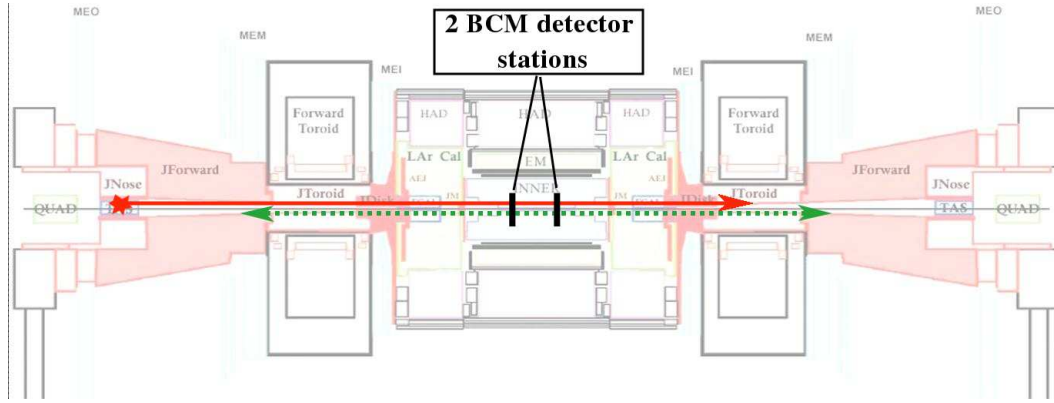
Figure 2: ATLAS detector with two BCM detector stations at \pm z_{bcm} . Shower particles (red) reach left stations z_{bcm}/c before interactions at the interaction point occur. Secondary particles from interactions (green) reach both stations z_{bcm}/c after interactions simultaneously.
