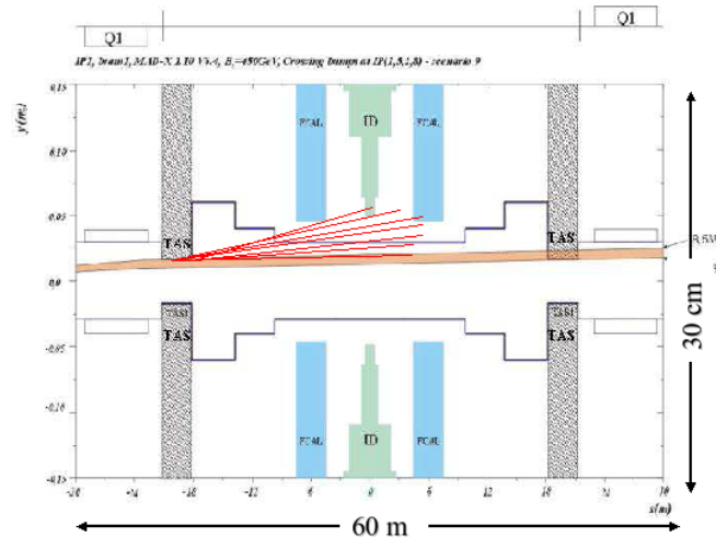
Figure 1: An example of a simulated beam accident in ATLAS[1] where proton beam hits the TAS collimators. The shaded region represents the range of beam directions dangerous for the Inner Detector. Red lines denote shower particles.
