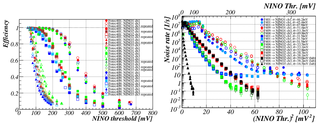
Figure 6: Measured NINO signal efficiency (left) and noise rate (right) dependence on NINO discriminator threshold measured with different prototype NINO boards (different markers) and various BCM detector modules (different colours) connected to them.
