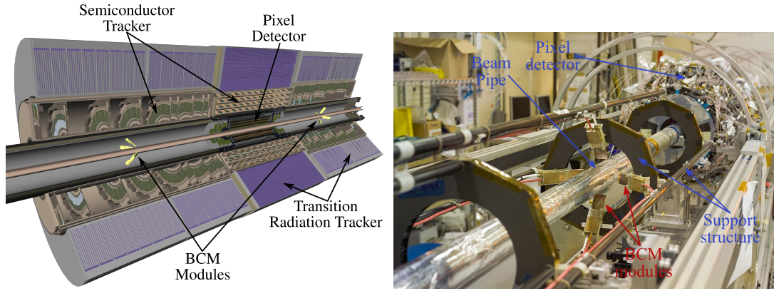
Figure 3: The BCM detector modules in their intended position inside the ATLAS Inner Detector (left), as visualised by the ATLAS event display VP1[3]. Modules are mounted on the Pixel support structure (right).
