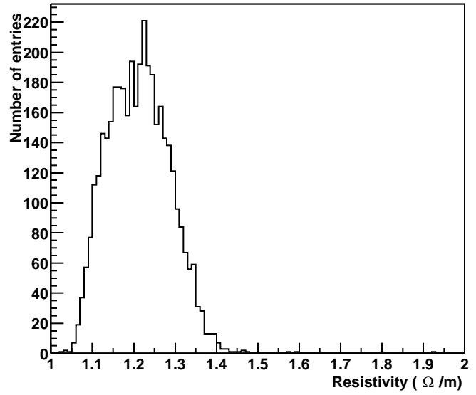
Resistivity of thin lines
