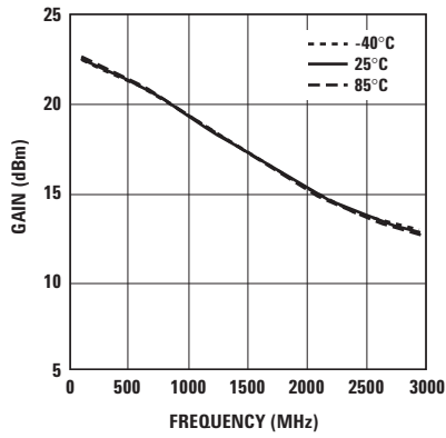
Figure 20. Gain vs. Frequency (5V 30 mA).
