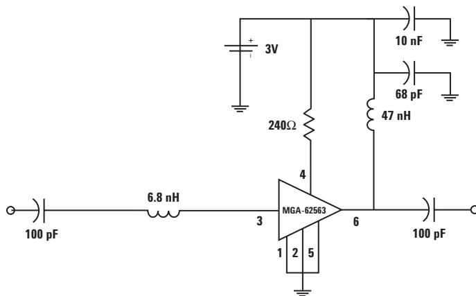
Figure 1. Test circuit of the 0.5 GHz production test board used for NF, Gain and OIP3 measurements. This circuit achieves a trade-off between optimal NF, Gain, OIP3 and input return loss. Circuit losses have been de-embedded from actual measurements.
